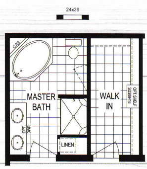
OPTIONAL DELUXE BATH (w/ CORNER DECK TUB) OPT. "A"
