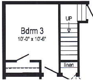
Optional Attic Stairs
